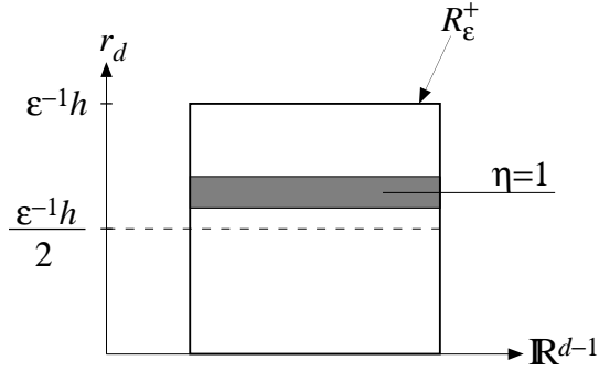
Fig.3. \mathcal{L}^{(1)}(m_\epsilon^{(3)}) = \mathcal{L}^*(m_\epsilon^{(3)}) = \emptyset , therefore \eta = 1 on \{\lambda(D) \geq n^* + 4\} . In particular \eta = 1 on the level \lambda(D) = n^* + 4 , which is shadowed. While the averages \pi_k m_\epsilon^{(3)} \geq m_\beta - \theta above this level, this may not be so point by point. However for the modification m_\epsilon^{(4)} of m_\epsilon^{(3)} , m_\epsilon^{(4)} \geq m_\beta - \theta on \{\lambda(D) > n^* + 4\} .
