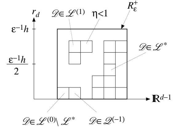
Fig.1. The cubes D \in \mathcal{Q}^{(-1)} \cap R_\varepsilon^+ where \eta < 1 . There are three clusters: the one on the upper left is in \mathcal{L}^{(1)} , the other two in \mathcal{L}^{(0)} ; the one on the bottom left is in \mathcal{L}^{(0)} \setminus \mathcal{L}^* the other one in \mathcal{L}^* , as its height exceeds \varepsilon^{-1}h/2 .
