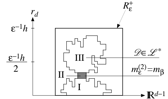
Fig.2. A cluster \mathcal{D} \in \mathcal{L}^*(m_\varepsilon^{(1)}) . \mathcal{D} is divided into three parts, I, II, and III. The shadowed region II is the minimal section of \mathcal{D} . The modification m_\varepsilon^{(2)} of m_\varepsilon^{(1)} is equal everywhere to m_\varepsilon^{(1)} except in II, where it has value m_\beta ; thus \eta_{m_\varepsilon^{(2)},k,\zeta} = 1 on II, hence III \in \mathcal{L}^{(1)}(m_\varepsilon^{(2)}) and I \in \mathcal{L}^{(0)}(m_\varepsilon^{(2)}) but I \notin \mathcal{L}^*(m_\varepsilon^{(2)}) , which is thus empty.
