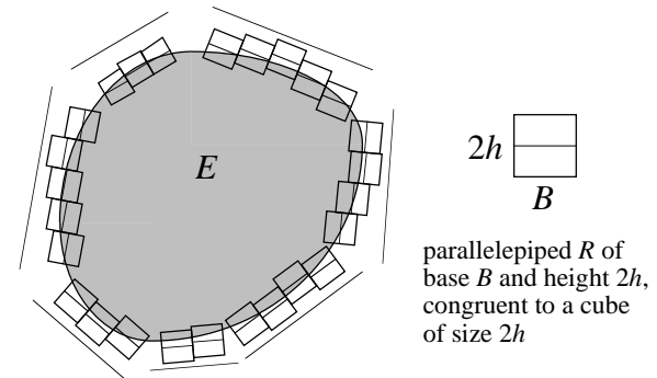
Fig.5. The shaded region is a set E with finite perimeter. Shown is a covering of parts of \partial E by parallelepipeds as in Theorem D.2. Locally \partial E is the graph of a function; the segments outside E represent symbolically the domains of definition of these functions.
