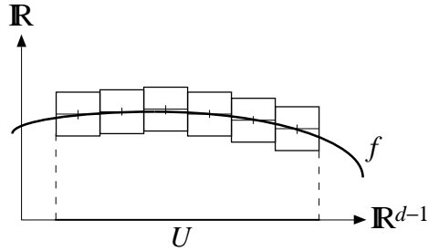
Fig.6. Blow up of a single piece of the covering of Fig. 5.
