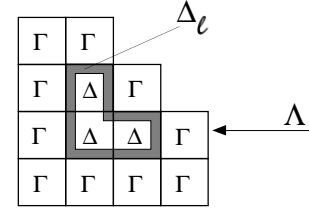
Fig.4. An example of the regions \Delta , \Gamma and \Lambda of Appendix B. \Delta is the union of the three central cubes, \Gamma of the ten cubes surrounding \Delta and \Lambda is the complement. The shadowed region represents \Delta_\ell .
