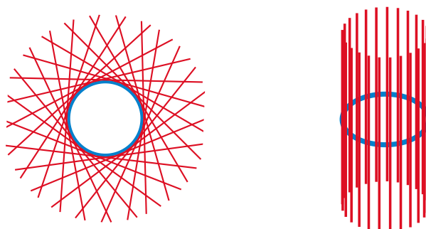
Figure 4.3. The tangent bundle of S^1 is trivial.
