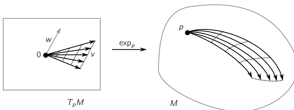
Figure 10.8. The family of curves used to prove the Gauss Lemma. Each \gamma_s is a geodesic exiting from p .
